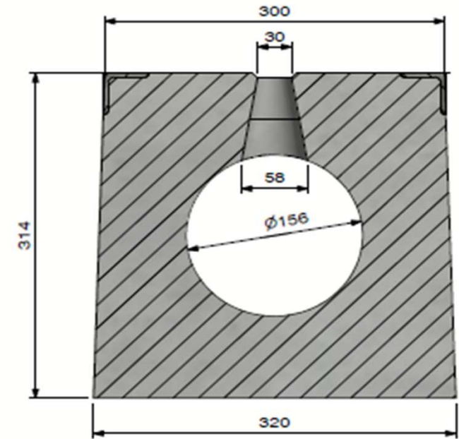
View B
