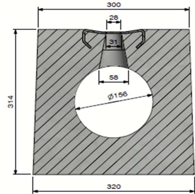
View B
