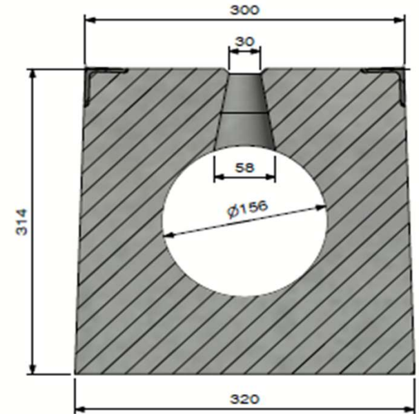
View B
