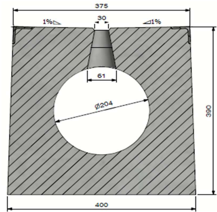
View B
