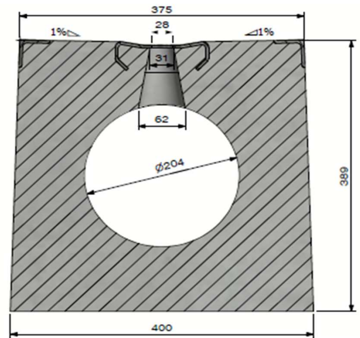
View B
