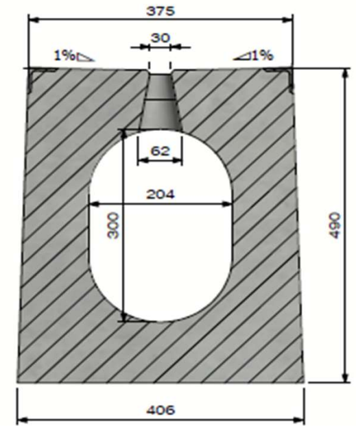
View B
