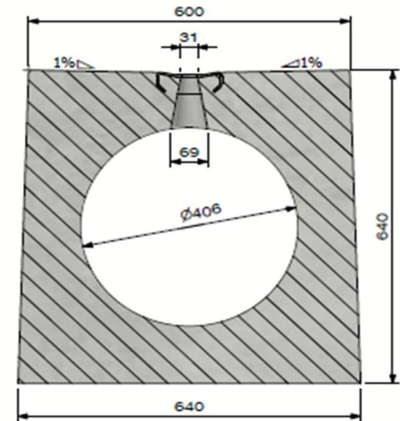
View B
