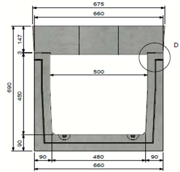
View B
